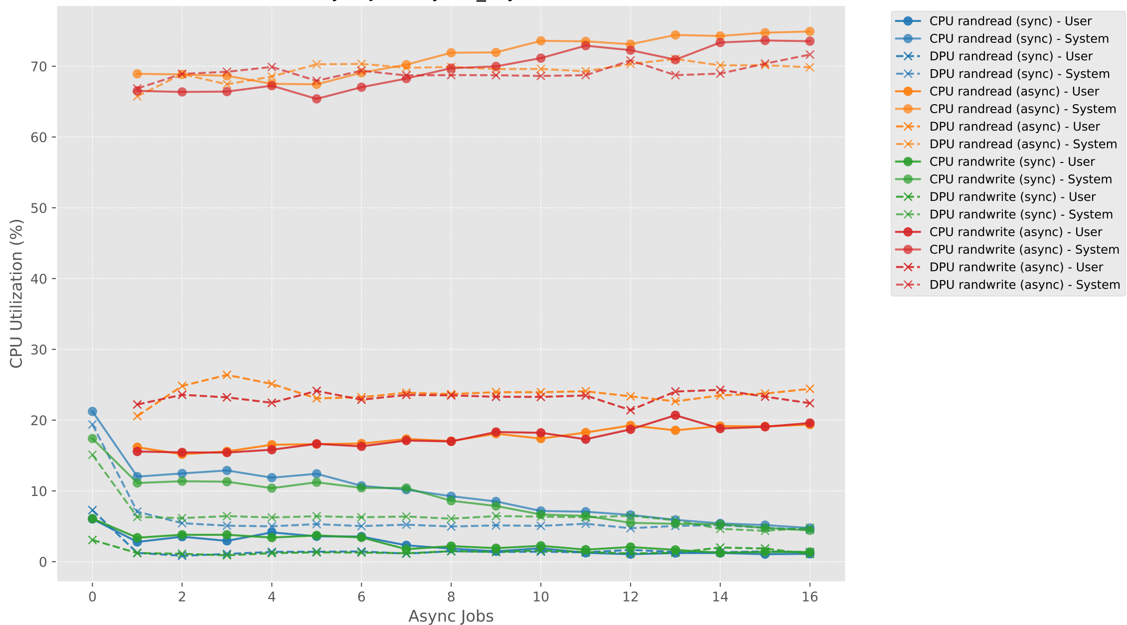
CPU Utilization vs Async Jobs (sync1_asyncN) - RAND (CPU vs DPU)
